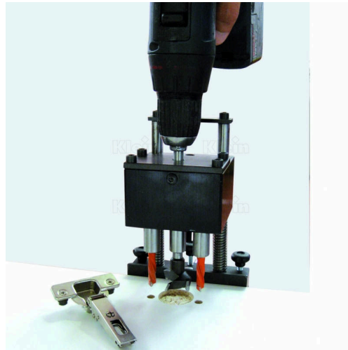
The central bit must have right hand rotation, the lateral bits have left hand rotation
