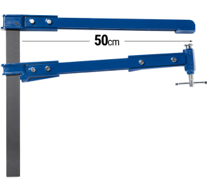
PIHER - Classic clamp Mod. 50K
