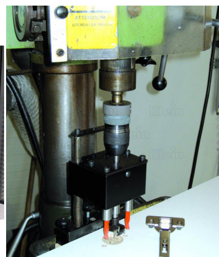
The central bit must have right hand rotation, the lateral bits have left hand rotation
