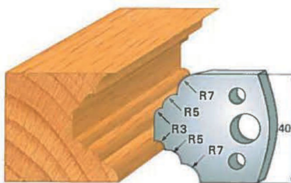
Art. SA0021 - (SA1021)
