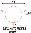
DRILL-MATIC TT52/5,5 Hettich
