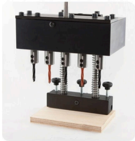
The central bit and those mounted in the external positions have right hand rotation, the other tools have left hand rotation.
