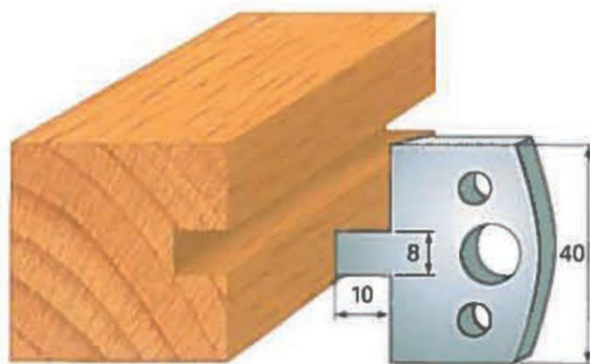
Art. SA0094 - (SA1094)
